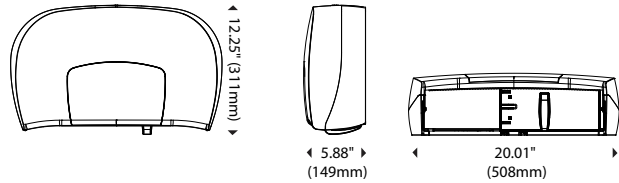
Dispenser Dimensions
