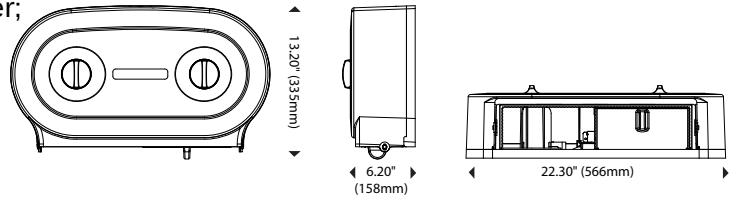
Dispenser Dimensions
